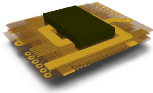
Figure 5.9 The final completely folded-up transformer, with 3D model of the Ferrrocube E18 ferrite magnetic core through the cutouts
